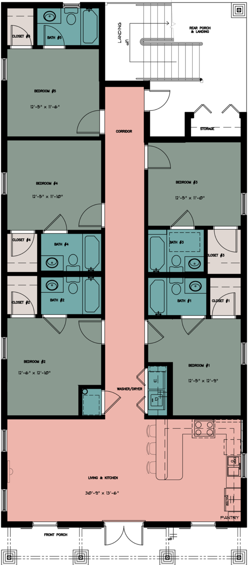
DUPLEX 1ST & 2ND FLOOR
